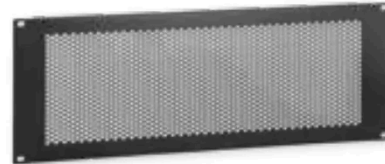
19" Vented Blank Panel, 4U [716321] Rackmount Spacer Panel with Perforated Venting, RAL 9005
